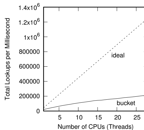
Figure 10.2: Read-Only Hash-Table Performance For Schrödinger's Zoo
