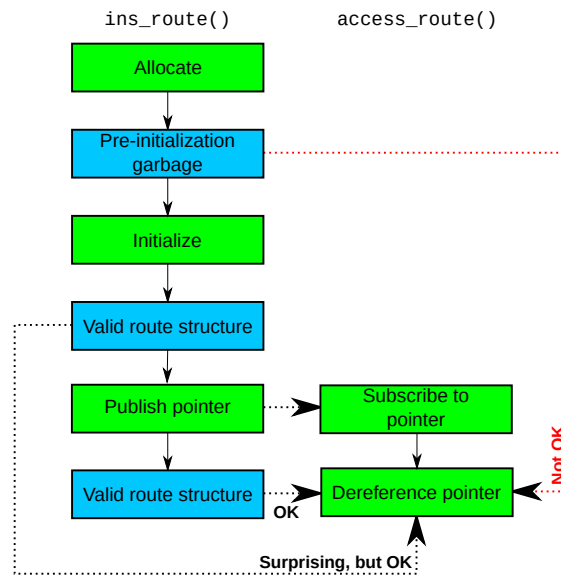
Figure 9.10: Publication/Subscription Constraints
