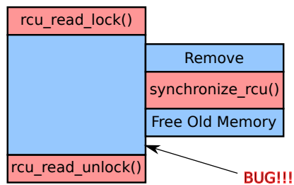
Figure 9.14: Summary of RCU Grace-Period Ordering Guarantees
