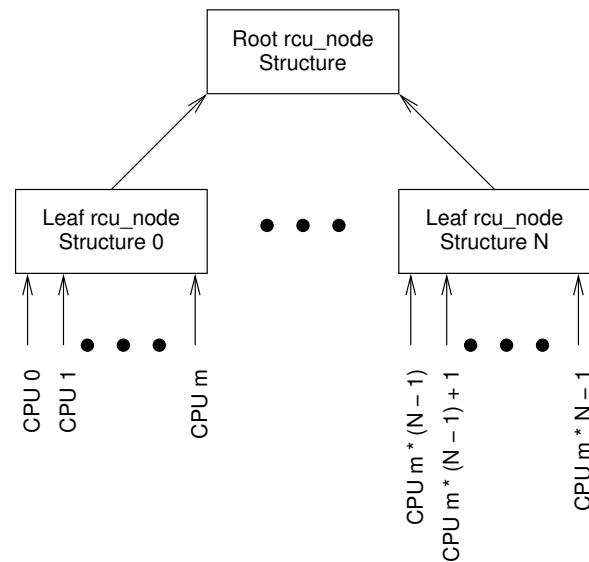
Figure 7.9: Locking Hierarchy
