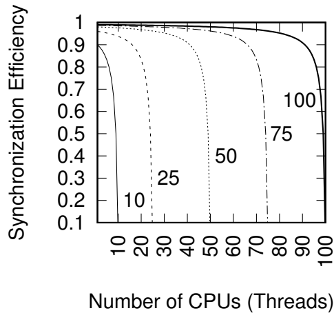
Figure 6.16: Synchronization Efficiency
